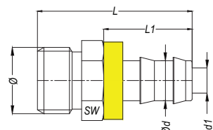
Male threaded push lock hose tail
