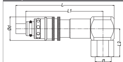
with female thread 90°
