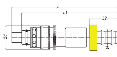
with push-lock hose tail
