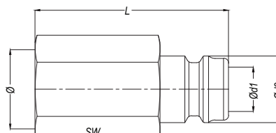
with female thread (090 serie)
