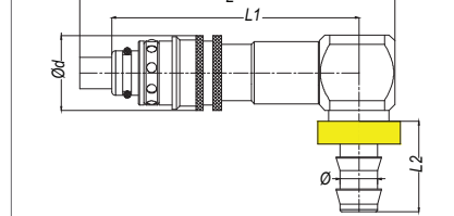
with push-lock hose tail 90°
