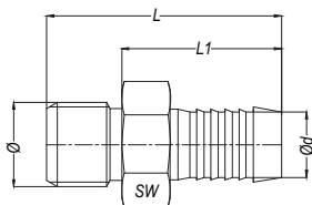
Male threaded hose tail
