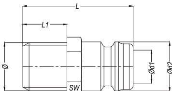
with male thread (090 serie)
