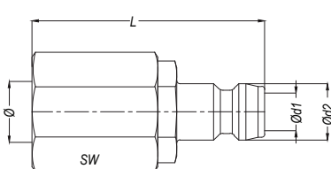
with female thread (060 serie)
