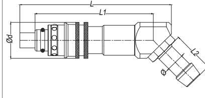
with female thread 45°
