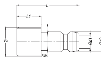
with male thread (060 serie)
