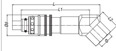
with female thread 45°
