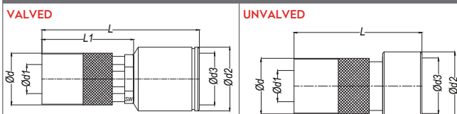
Adapting Socket with 100.08 Plug
