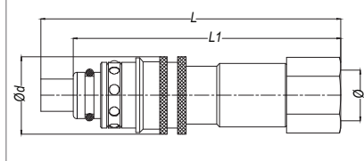
with female thread
