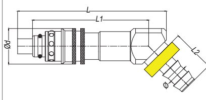
with push-lock hose tail 45°
