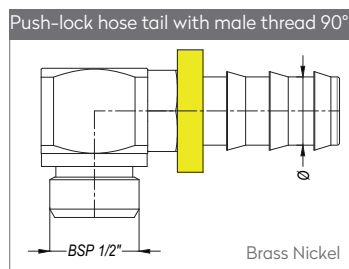
Push-lock hose tail with male thread 90°
