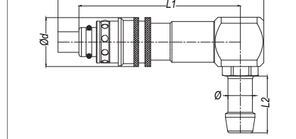
with female thread 90°
