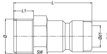
with male thread (190 serie)
